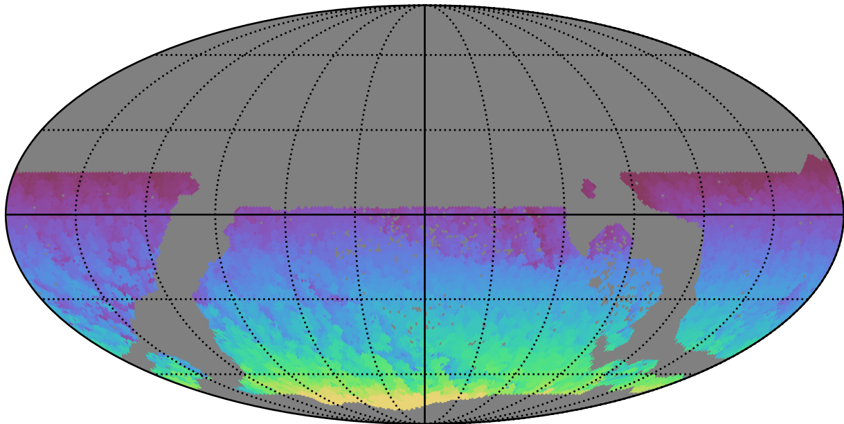
ddf_acor_sf25_lsf40_lsr10_v3.4_10yrs WFD all bands: Max HA
