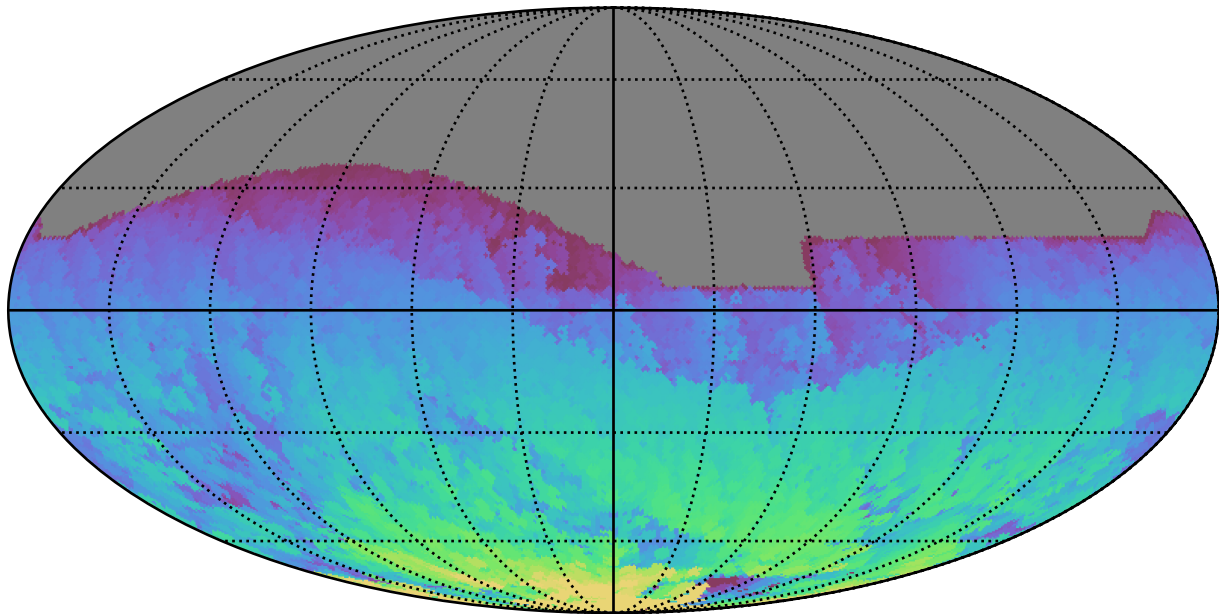
ddf_acor_sf25_lsf40_lsr10_v3.4_10yrs All sky z band: Max HA
