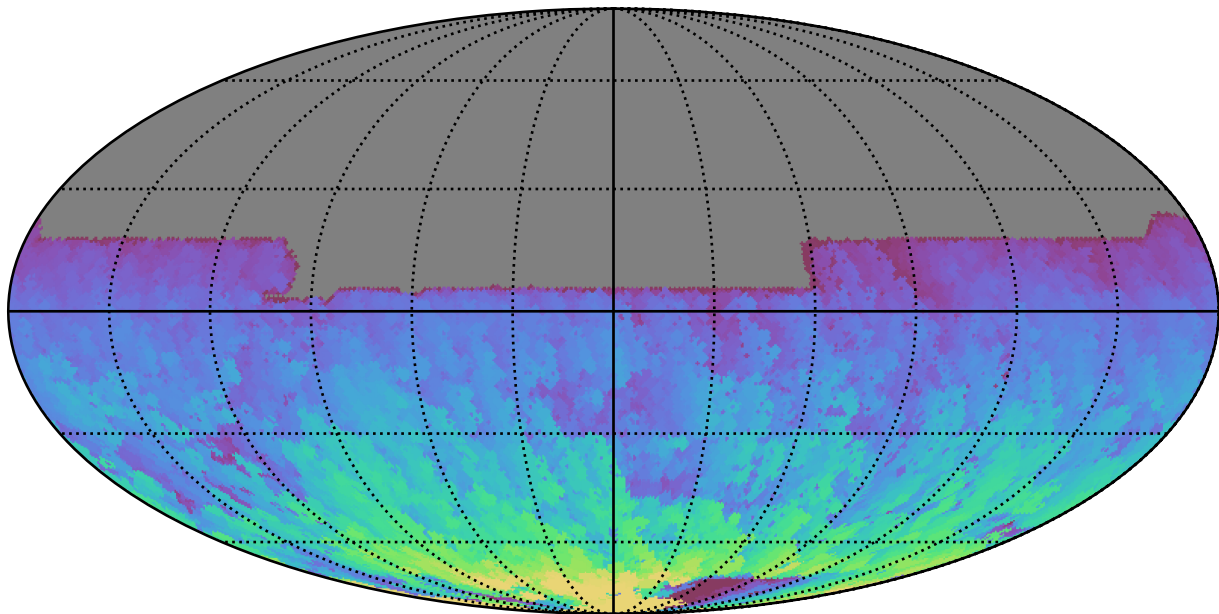
ddf_acor_sf25_lsf40_lsr10_v3.4_10yrs All sky y band: Max HA
