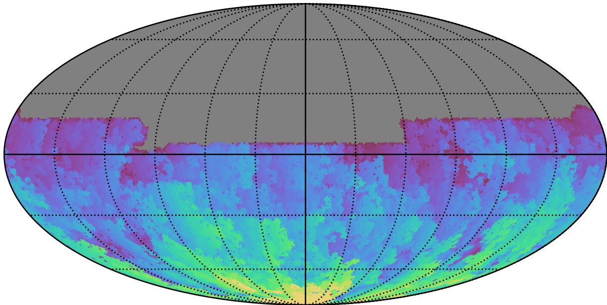
ddf_acor_sf25_lsf40_lsr10_v3.4_10yrs All sky u band: Max HA
