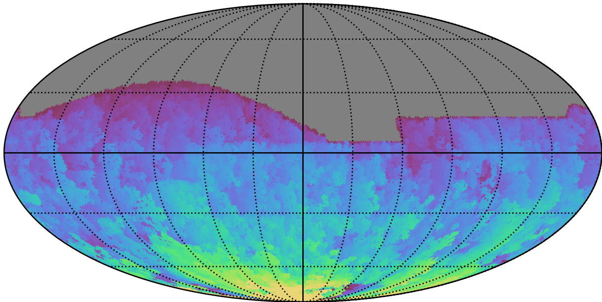
ddf_acor_sf25_lsf40_lsr10_v3.4_10yrs All sky r band: Max HA
