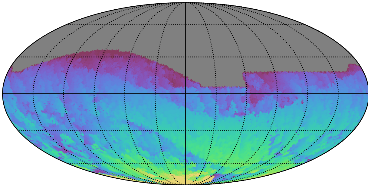
ddf_acor_sf25_lsf40_lsr10_v3.4_10yrs All sky i band: Max HA
