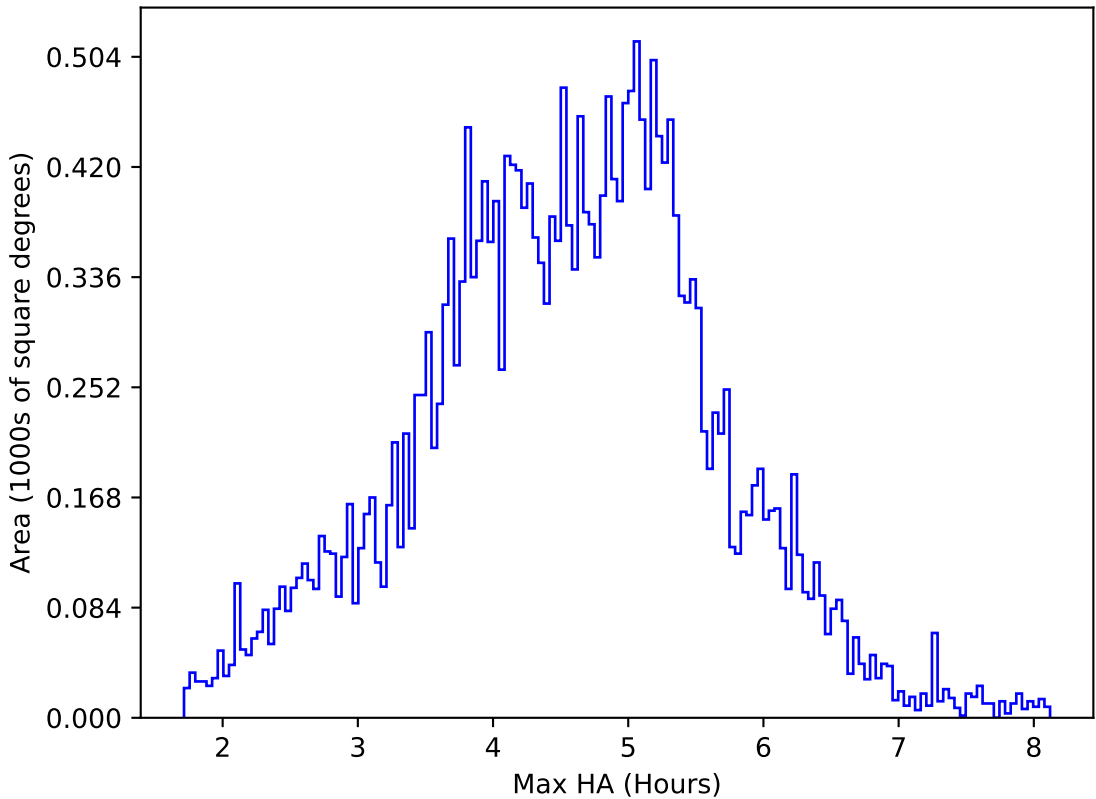
ddf_acor_sf25_lsf40_lsr10_v3.4_10yrs All sky i band: Max HA
