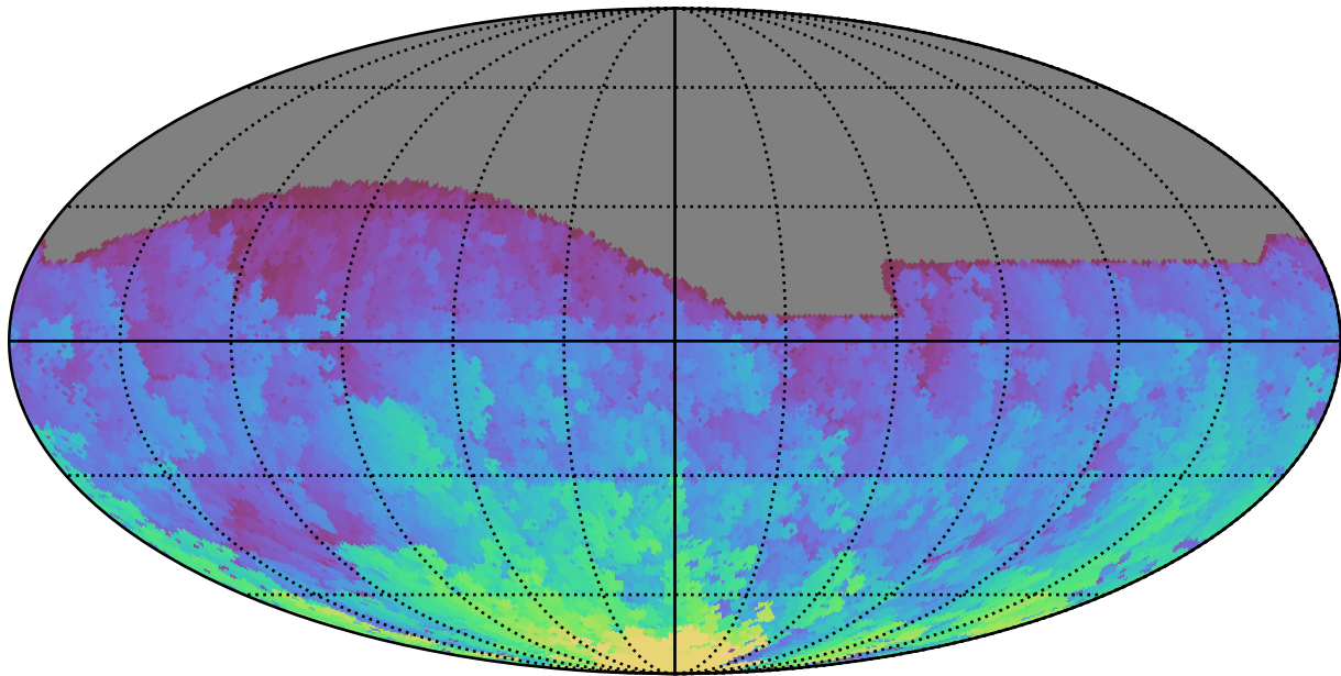
ddf_acor_sf25_lsf40_lsr10_v3.4_10yrs All sky g band: Max HA
