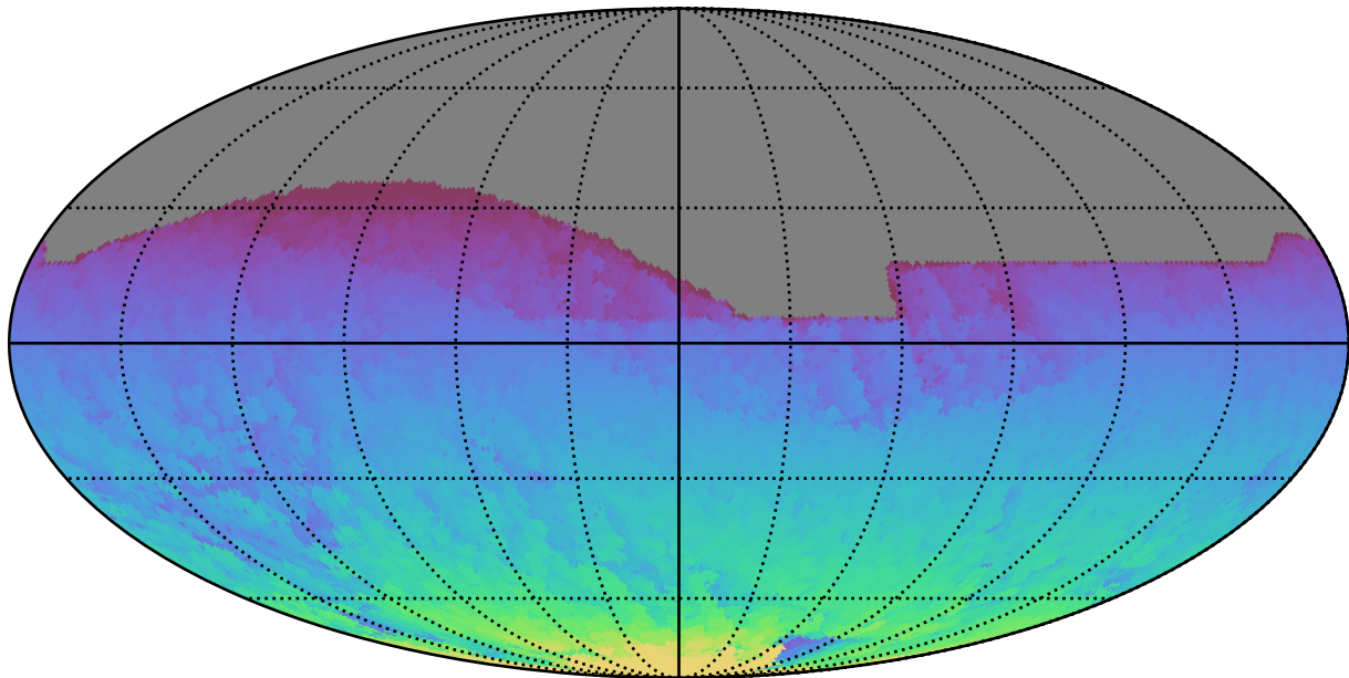
ddf_acor_sf25_lsf40_lsr10_v3.4_10yrs All sky all bands: Max HA
