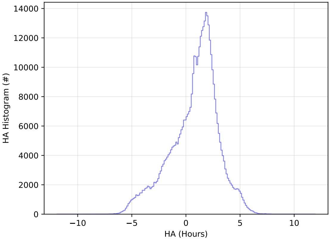
ddf_acor_sf25_lsf40_lsr10_v3.4_10yrs WFD z band: HA Histogram
