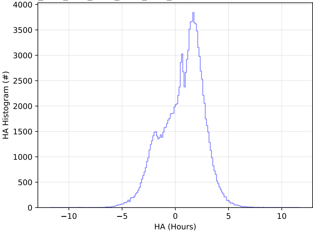
ddf_acor_sf25_lsf40_lsr10_v3.4_10yrs WFD u band: HA Histogram
