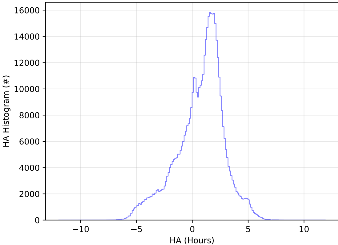
ddf_acor_sf25_ls40_lsr10_v3.4_10yrs WFD i band: HA Histogram
