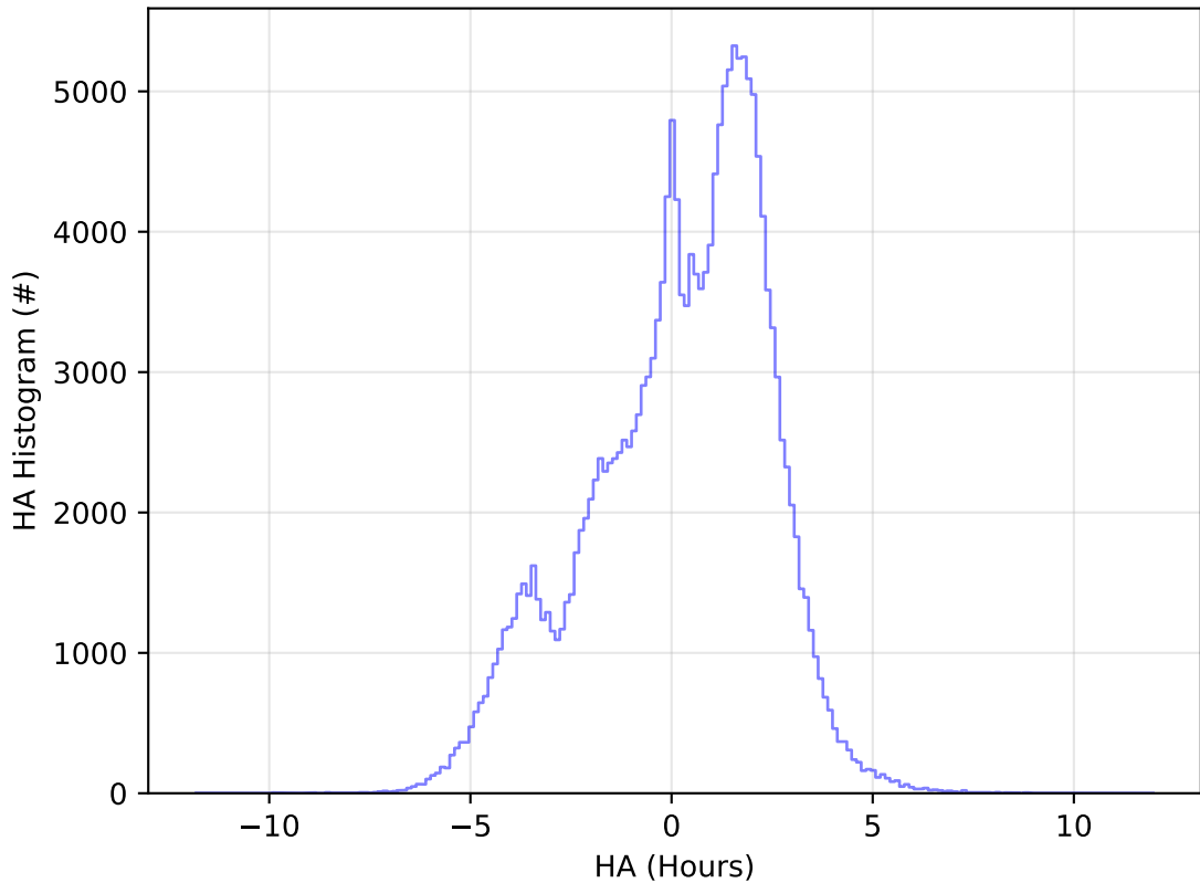
ddf_acor_sf25_lsf40_lsr10_v3.4_10yrs WFD g band: HA Histogram
