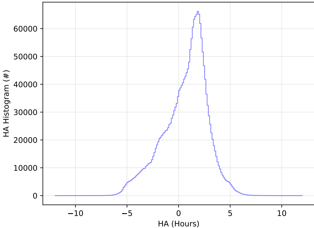
ddf_acor_sf25_lsf40_lsr10_v3.4_10yrs WFD all bands: HA Histogram
