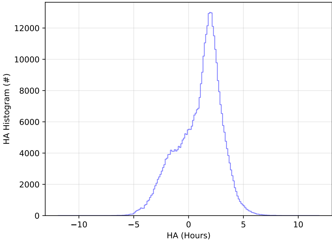
ddf_acor_sf25_lsf40_lsr10_v3.4_10yrs All sky y band: HA Histogram
