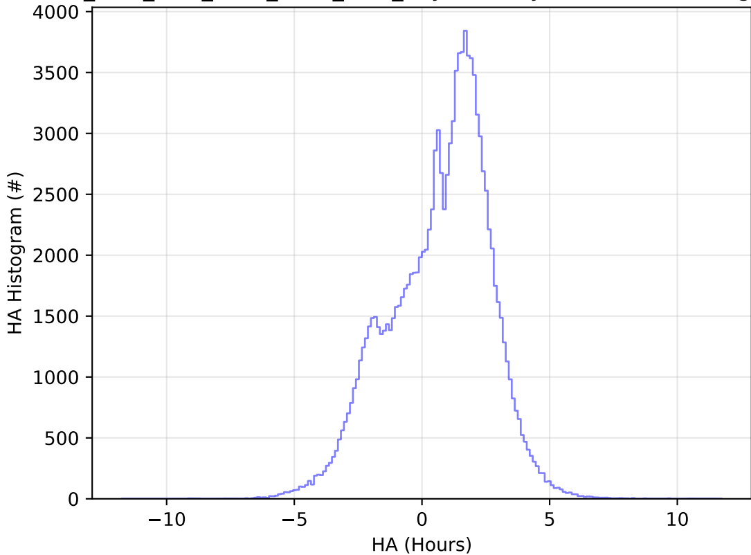
ddf_acor_sf25_lsf40_lsr10_v3.4_10yrs All sky u band: HA Histogram
