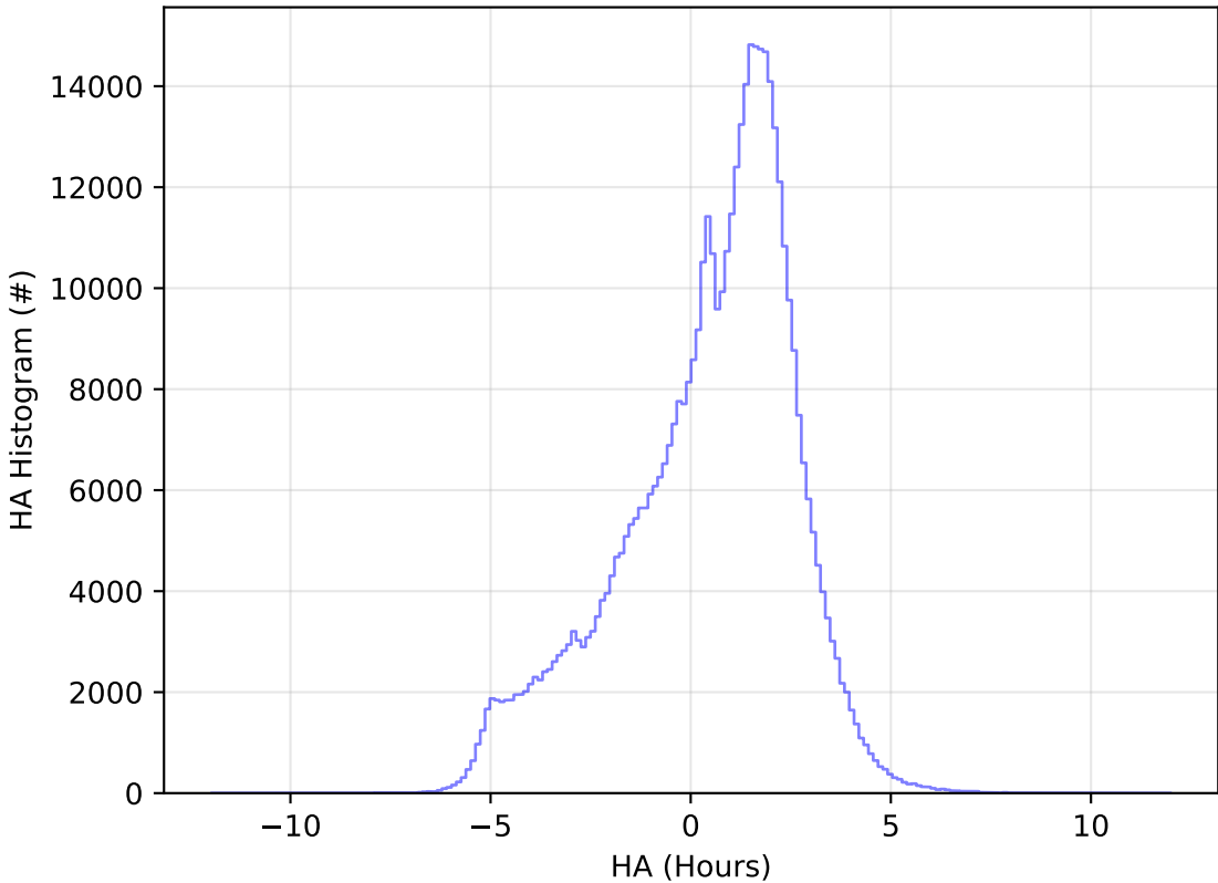
ddf_acor_sf25_lsf40_lsr10_v3.4_10yrs All sky r band: HA Histogram
