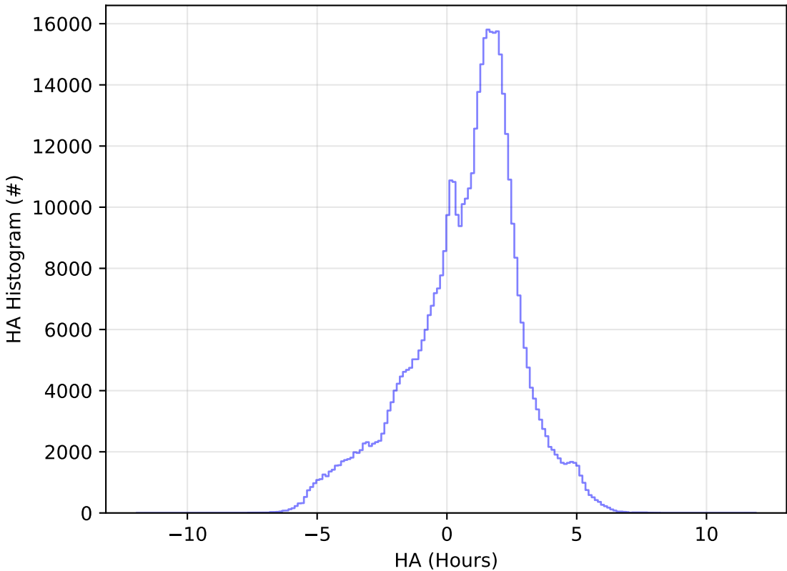
ddf_acor_sf25_lsf40_lsr10_v3.4_10yrs All sky i band: HA Histogram
