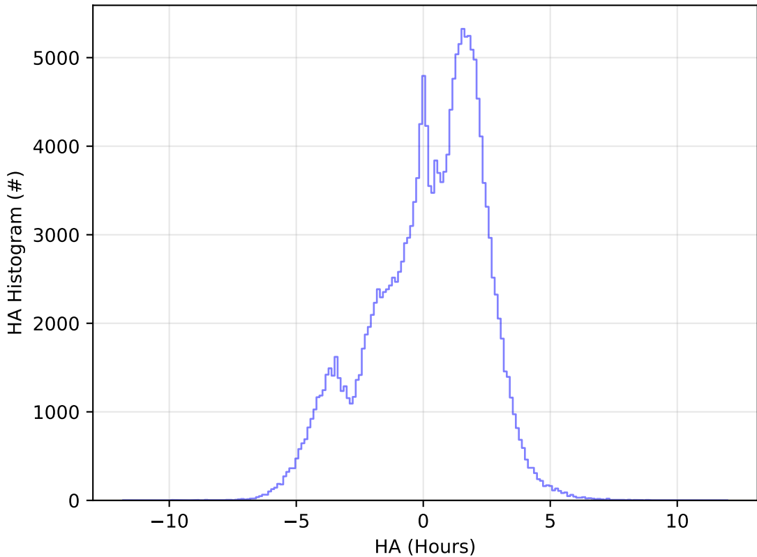
ddf_acor_sf25_lsf40_lsr10_v3.4_10yrs All sky g band: HA Histogram
