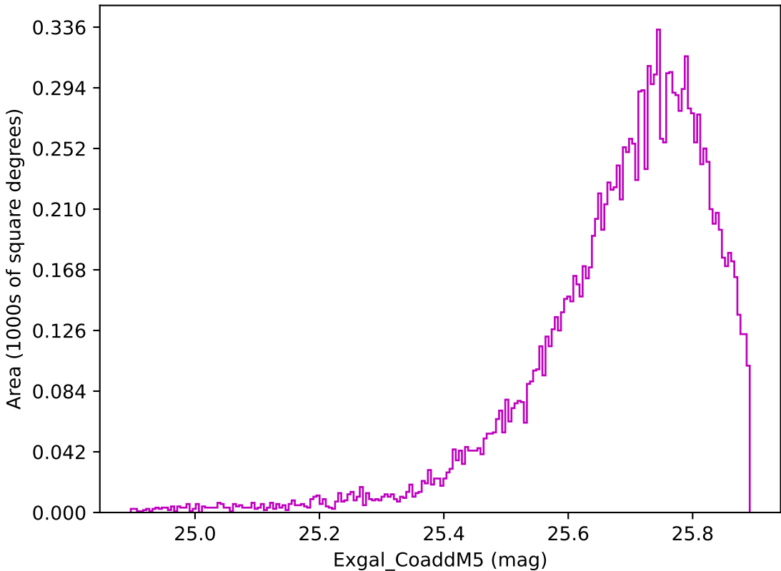
ddf_acor_sf25_lsf40_lsr10_v3.4_10yrs WFD z band: Exgal_CoaddM5
