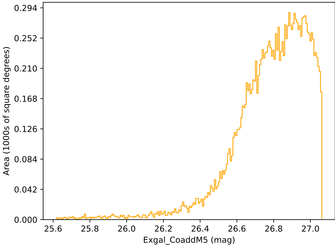
ddf_acor_sf25_lsf40_lsr10_v3.4_10yrs WFD r band: Exgal_CoaddM5
