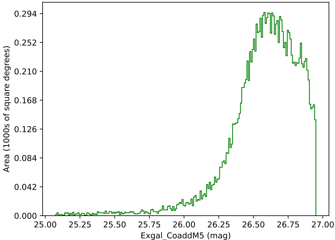
ddf_acor_sf25_lsf40_lsr10_v3.4_10yrs WFD g band: Exgal_CoaddM5
