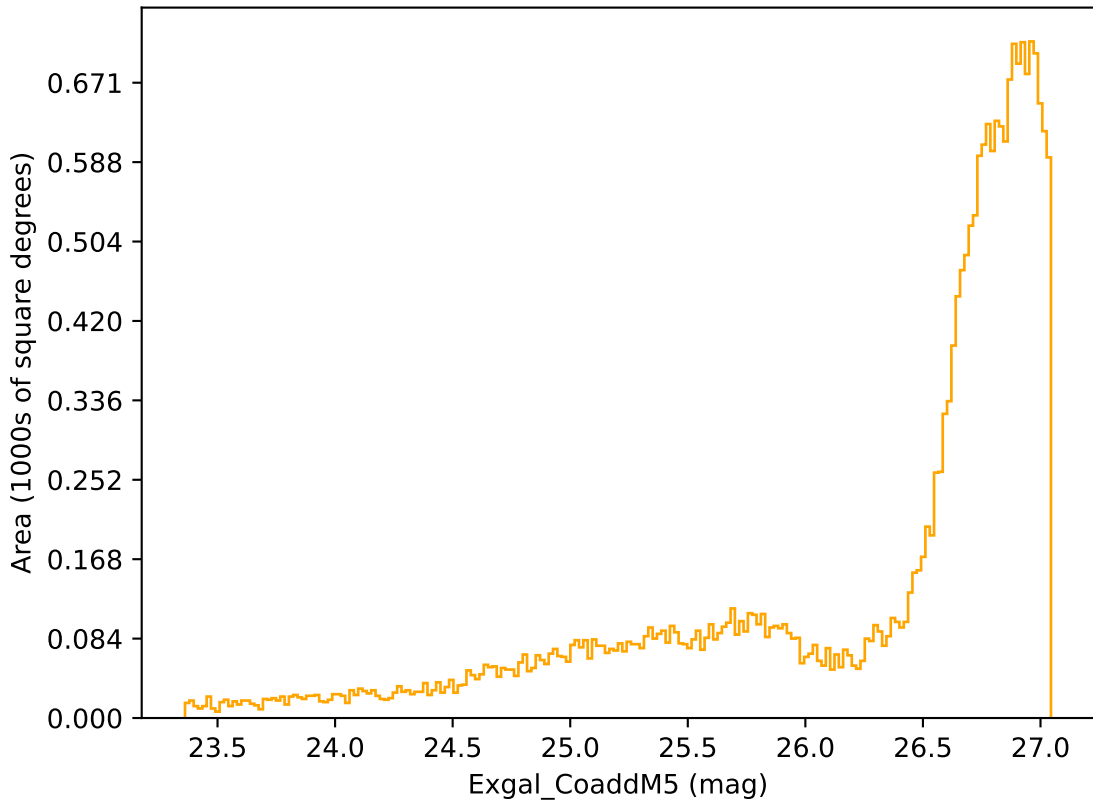
ddf_acor_sf25_lsf40_lsr10_v3.4_10yrs All sky r band: Exgal_CoaddM5
