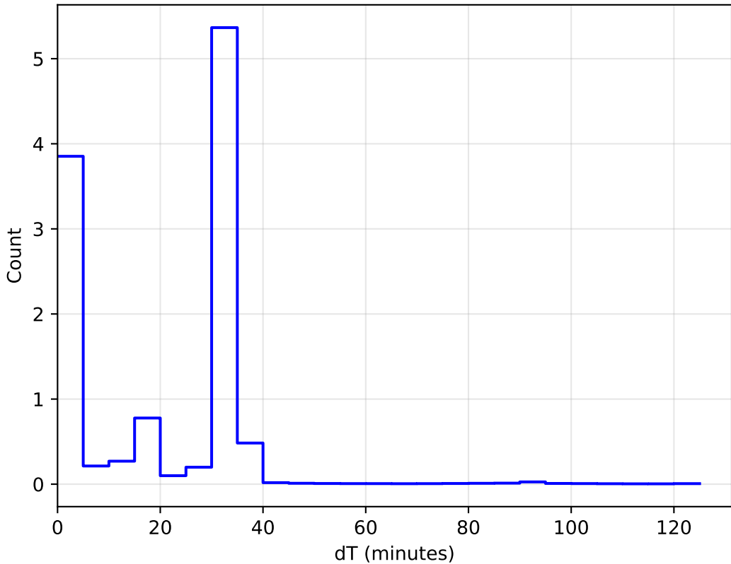
ddf_acor_sf25_lsf40_lsr10_v3.4_10yrs WFD: DeltaT Histogram 1e6
