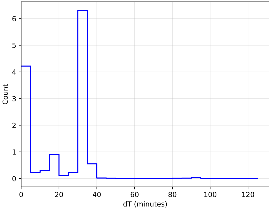
ddf_acor_sf25_lsf40_lsr10_v3.4_10yrs All sky: DeltaT Histogram
