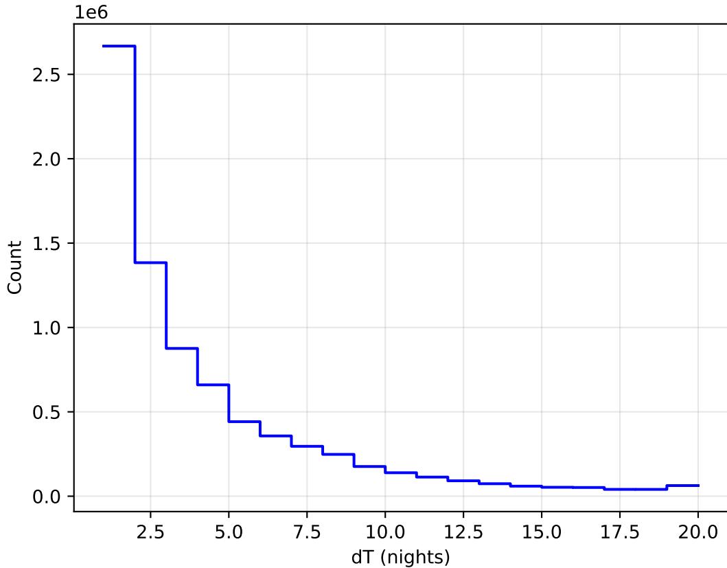
ddf_acor_sf25_lsf40_lsr10_v3.4_10yrs WFD all bands: DeltaNight Histogram
