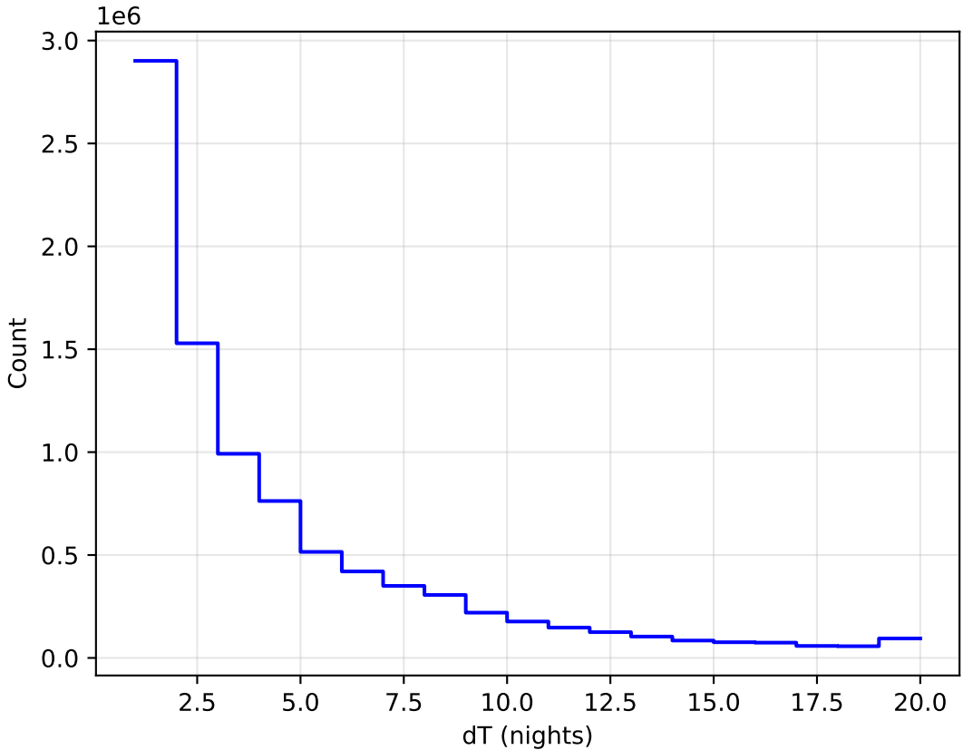
ddf_acor_sf25_lsf40_lsr10_v3.4_10yrs All sky all bands: DeltaNight Histogram
