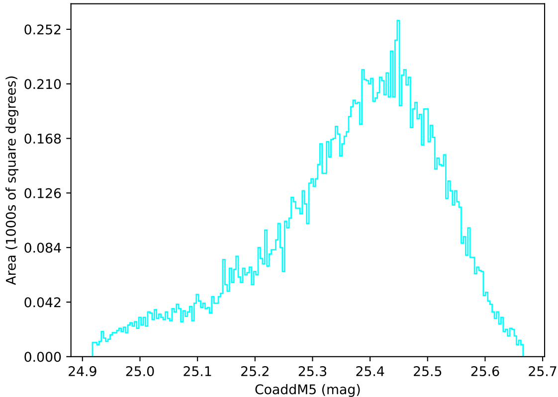
ddf_acor_sf25_lsf40_lsr10_v3.4_10yrs WFD u band: CoaddM5
