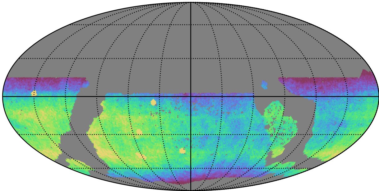
ddf_acor_sf25_lsf40_lsr10_v3.4_10yrs WFD r band: CoaddM5
