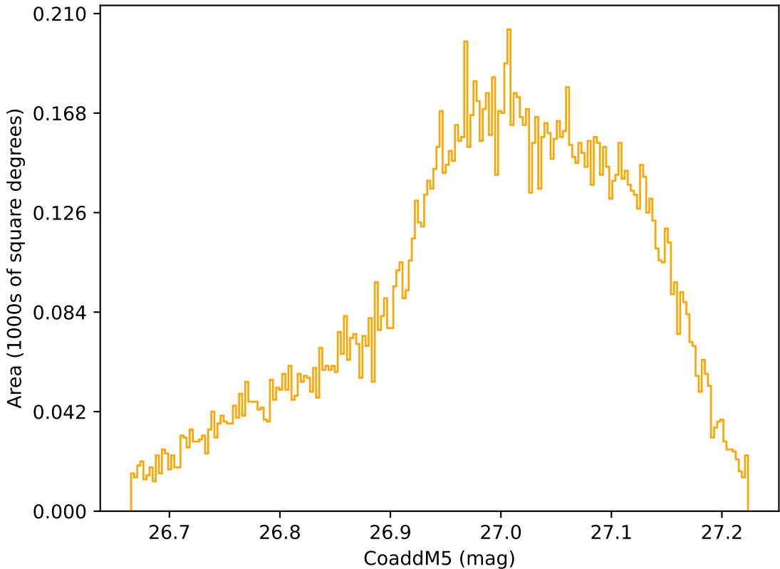
ddf_acor_sf25_lsf40_lsr10_v3.4_10yrs WFD r band: CoaddM5
