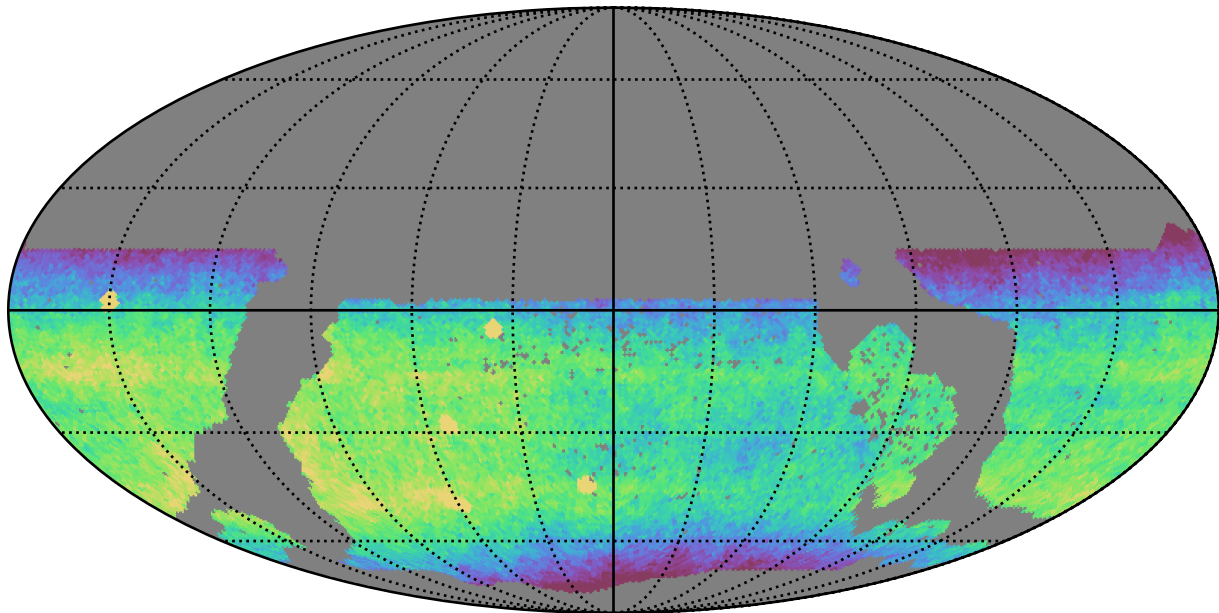
ddf_acor_sf25_lsf40_lsr10_v3.4_10yrs WFD i band: CoaddM5
