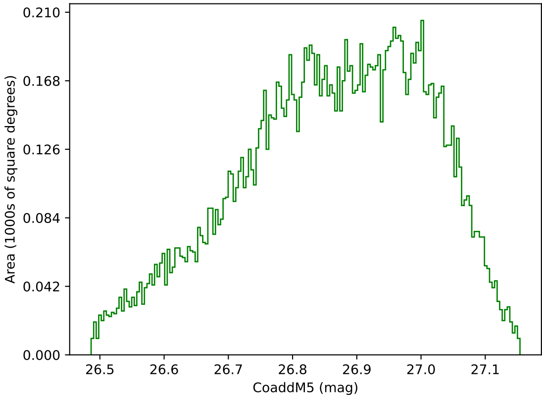
ddf_acor_sf25_lsf40_lsr10_v3.4_10yrs WFD g band: CoaddM5
