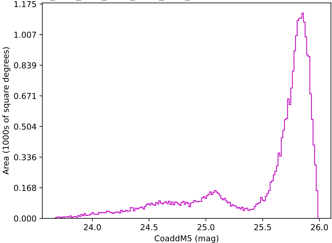
ddf_acor_sf25_lsf40_lsr10_v3.4_10yrs All sky z band: CoaddM5
