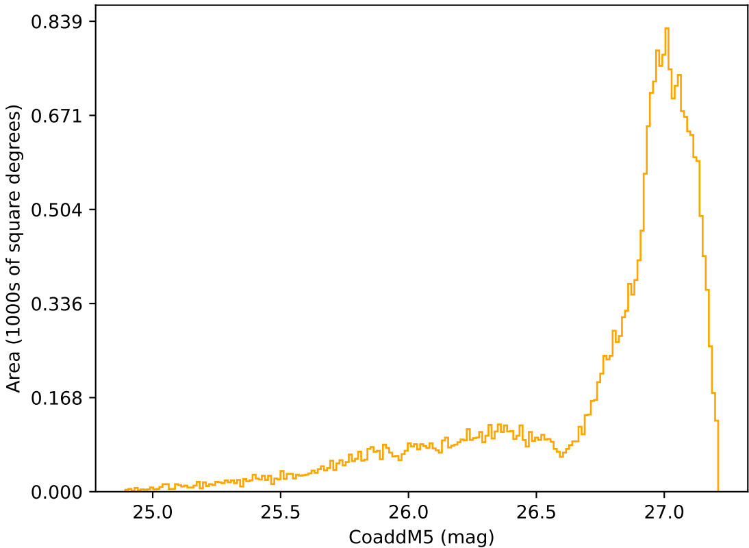
ddf_acor_sf25_lsf40_lsr10_v3.4_10yrs All sky r band: CoaddM5
