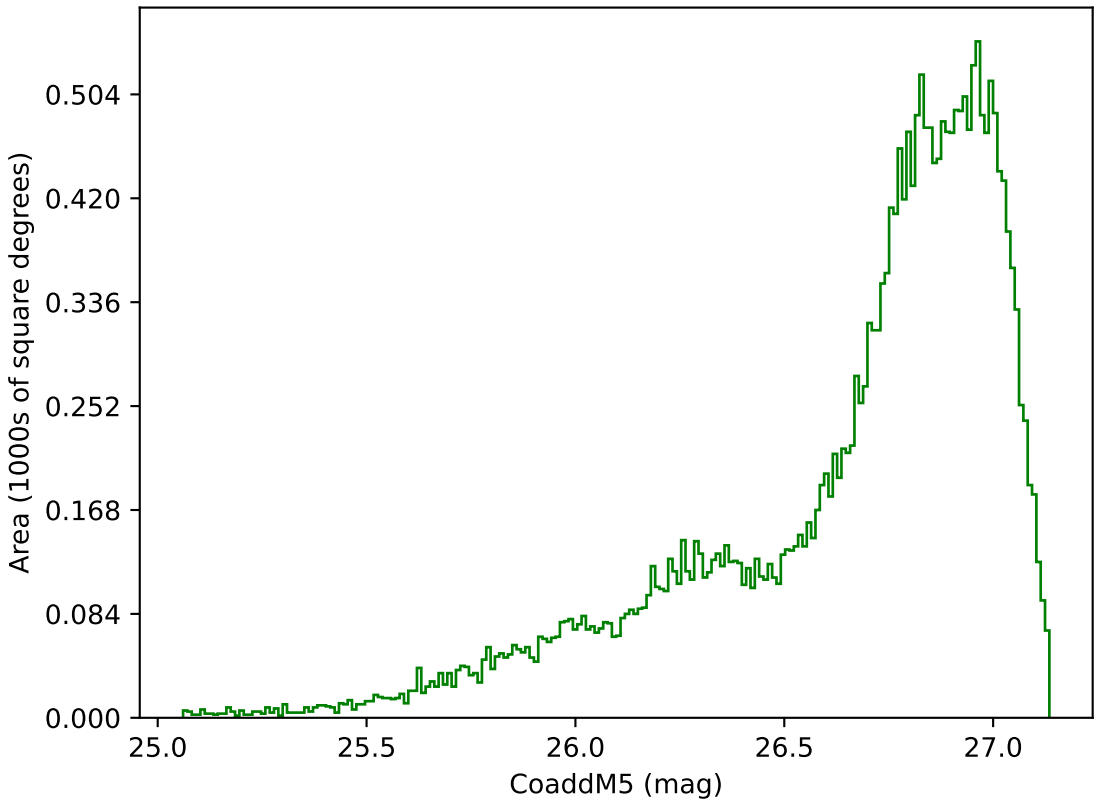
ddf_acor_sf25_lsf40_lsr10_v3.4_10yrs All sky g band: CoaddM5
