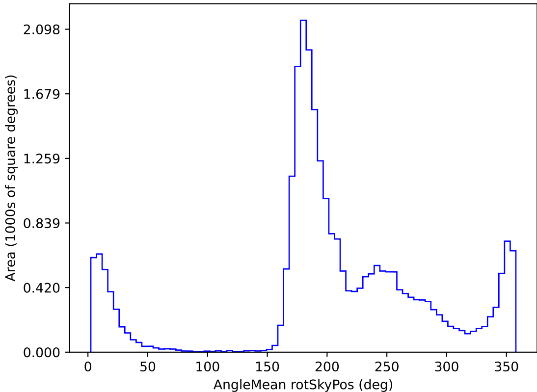
ddf_acor_sf25_lsf40_lsr10_v3.4_10yrs All sky i band: AngleMean rotSkyPos
