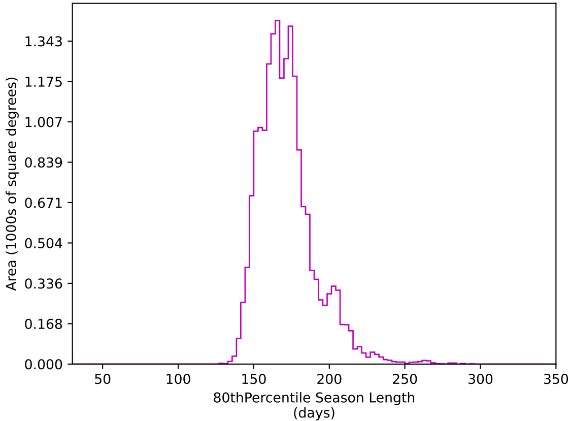
ddf_acor_sf25_lsf40_lsr10_v3.4_10yrs WFD z band: 80thPercentile Season Length
