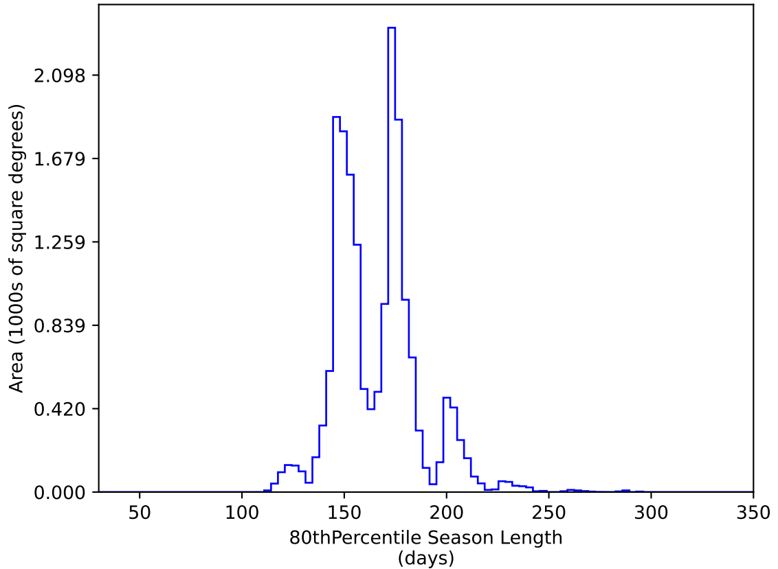
ddf_acor_sf25_lsf40_lsr10_v3.4_10yrs WFD y band: 80thPercentile Season Length
