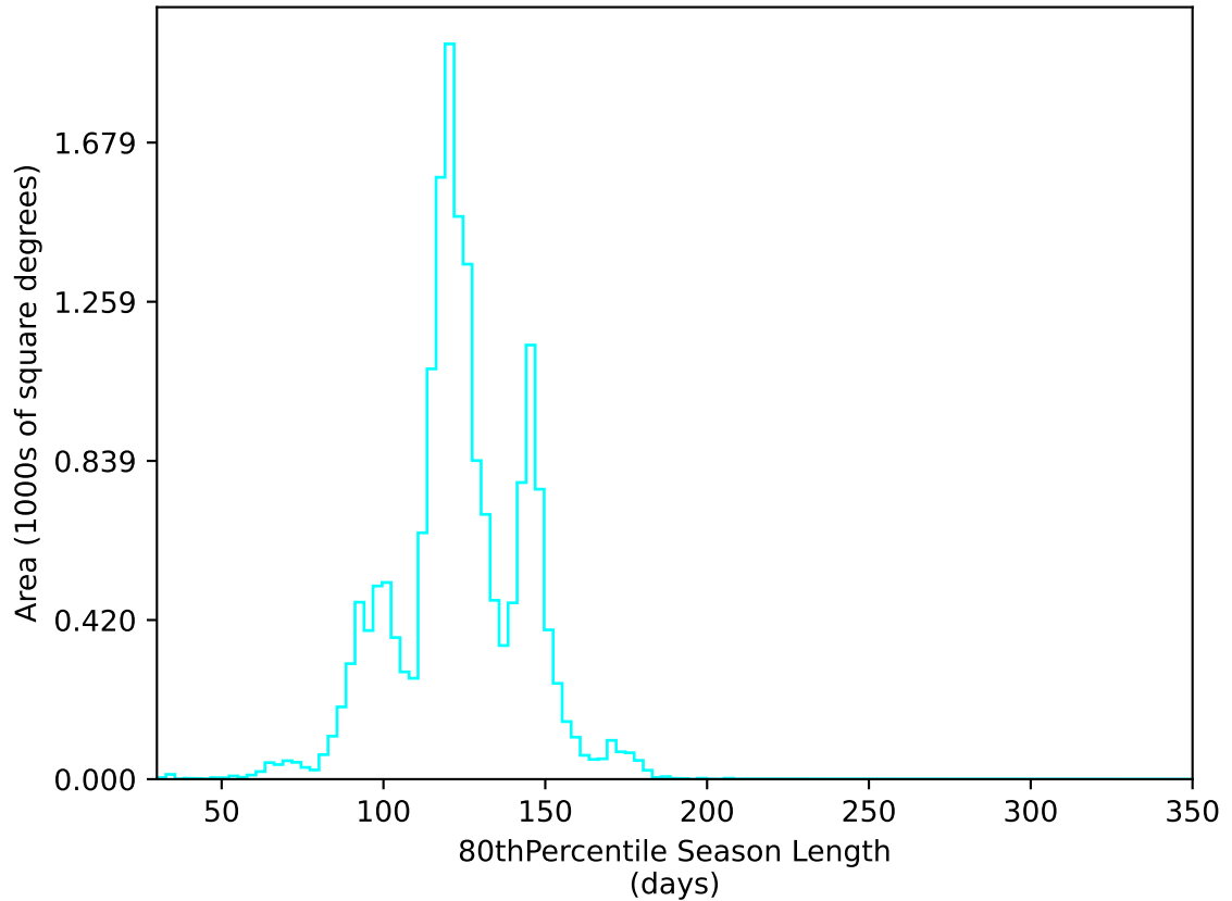
ddf_acor_sf25_lsf40_lsr10_v3.4_10yrs WFD u band: 80thPercentile Season Length
