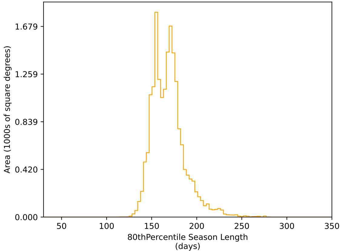
ddf_acor_sf25_lsf40_lsr10_v3.4_10yrs WFD r band: 80thPercentile Season Length
