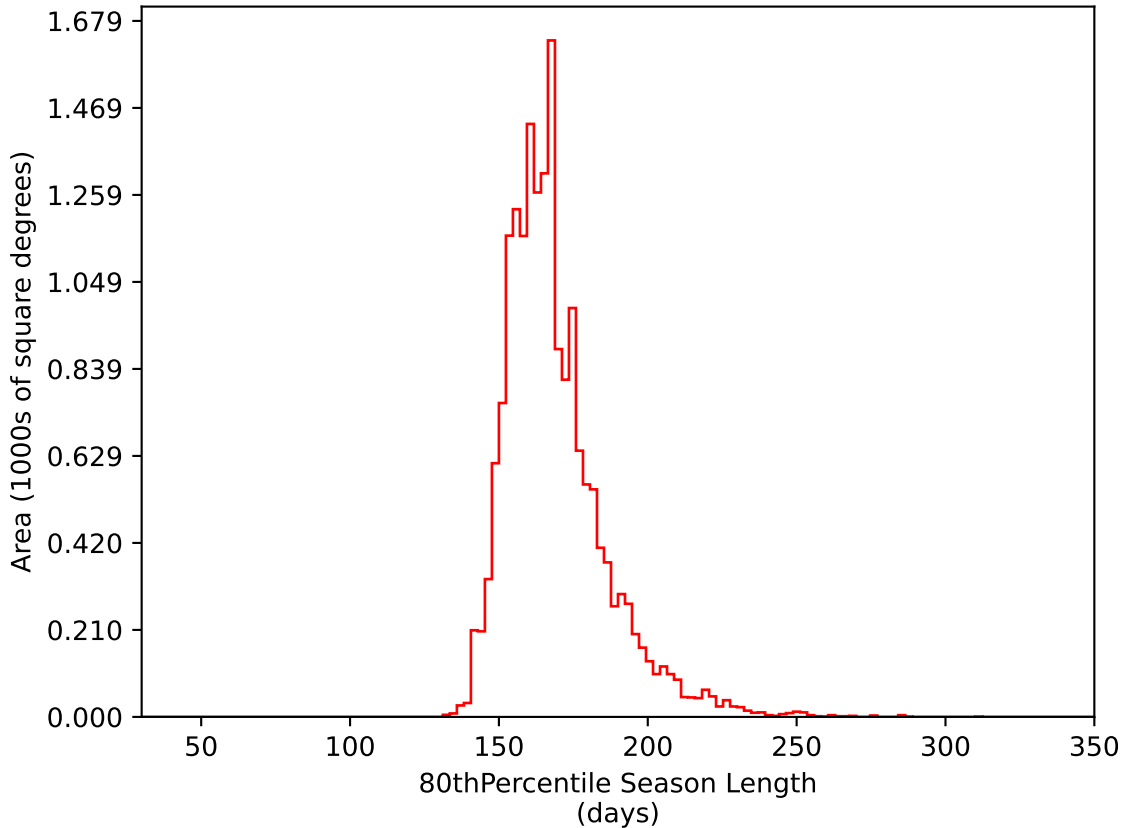
ddf_acor_sf25_lsf40_lsr10_v3.4_10yrs WFD i band: 80thPercentile Season Length
