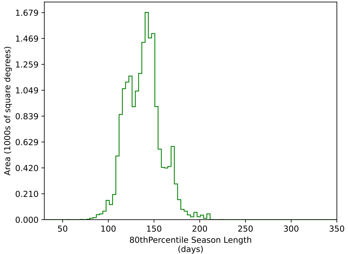
ddf_acor_sf25_lsf40_lsr10_v3.4_10yrs WFD g band: 80thPercentile Season Length
