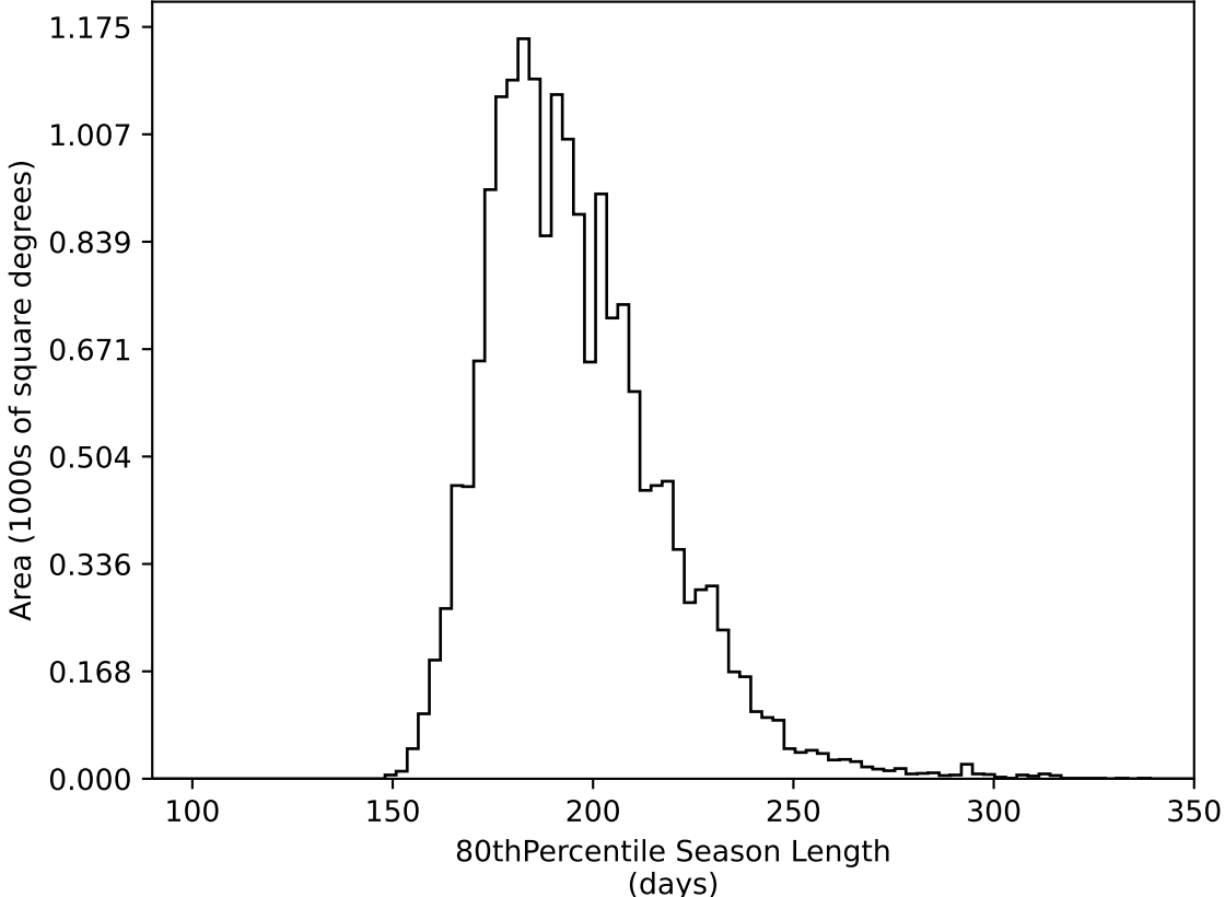
ddf_acor_sf25_lsf40_lsr10_v3.4_10yrs WFD all bands: 80thPercentile Season Length
