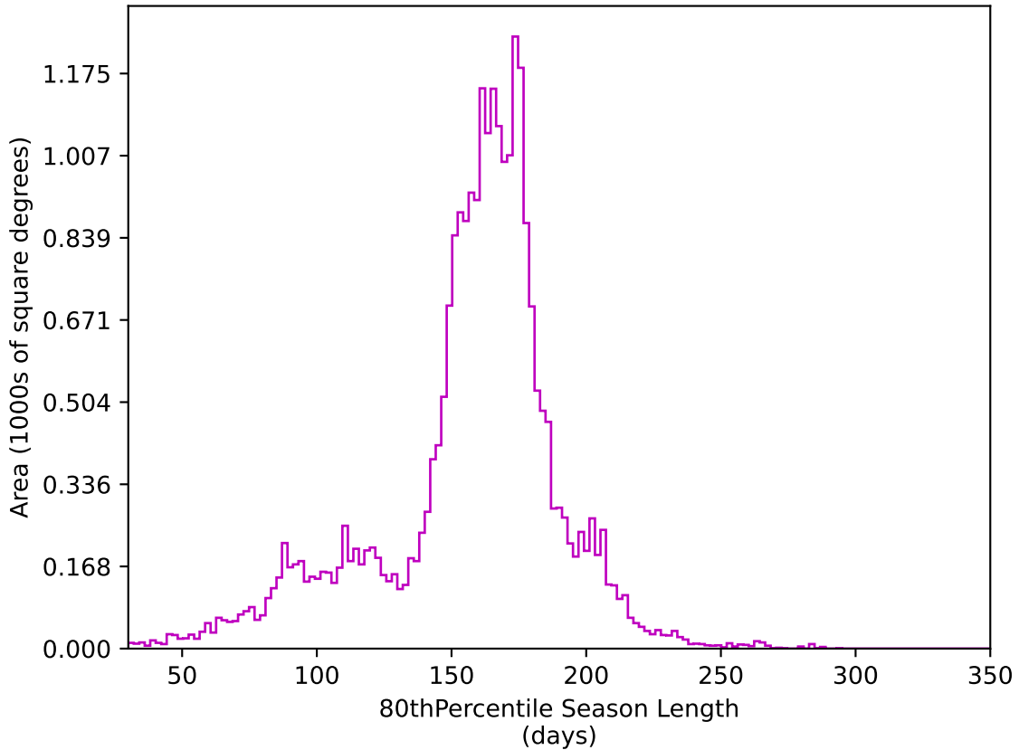
ddf_acor_sf25_lsf40_lsr10_v3.4_10yrs All sky z band: 80thPercentile Season Length
