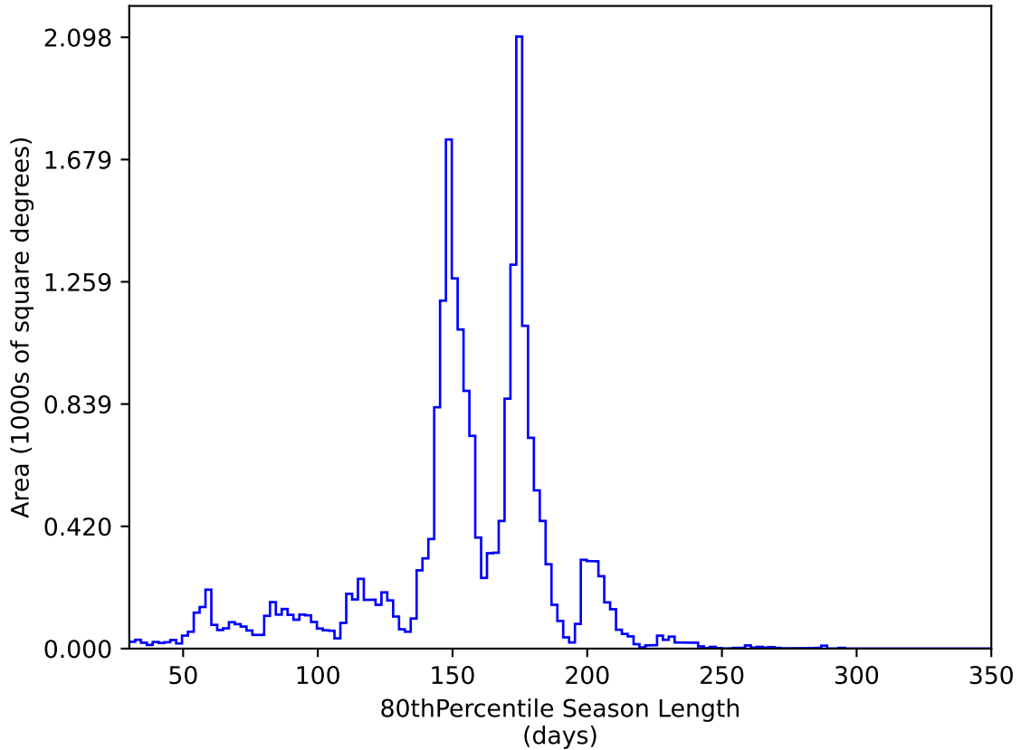
ddf_acor_sf25_lsf40_lsr10_v3.4_10yrs All sky y band: 80thPercentile Season Length
