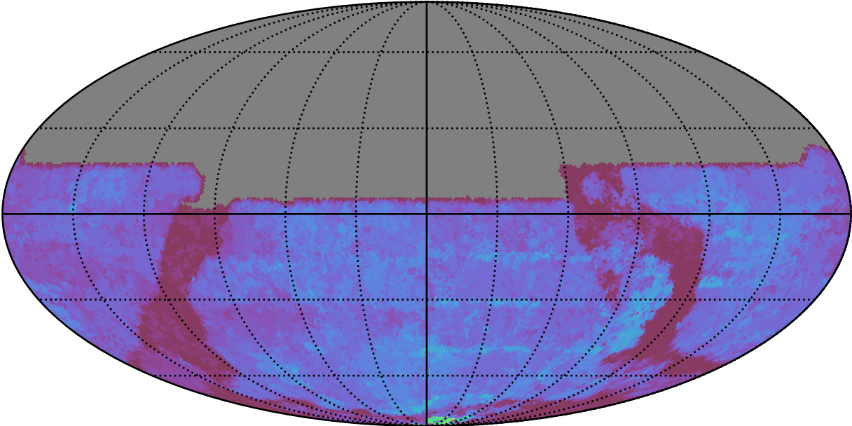
ddf_acor_sf25_lsf40_lsr10_v3.4_10yrs All sky u band: 80thPercentile Season Length
