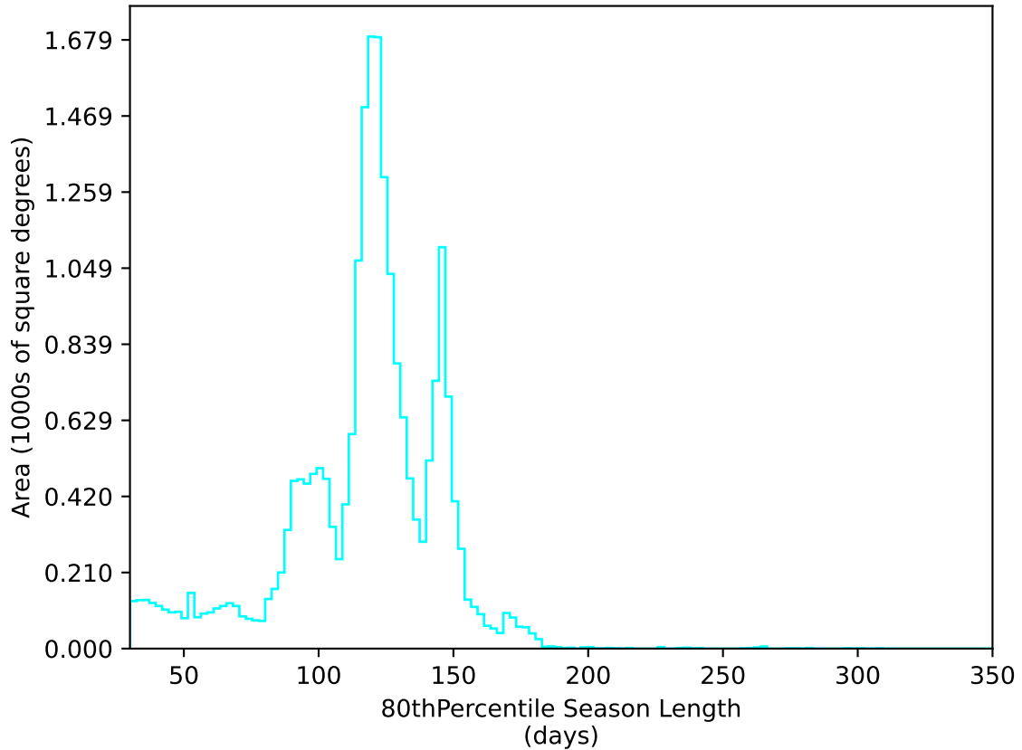
ddf_acor_sf25_lsf40_lsr10_v3.4_10yrs All sky u band: 80thPercentile Season Length
