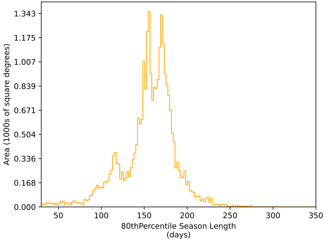
ddf_acor_sf25_lsf40_lsr10_v3.4_10yrs All sky r band: 80thPercentile Season Length
