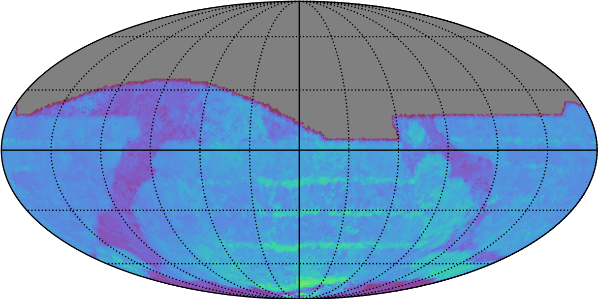
ddf_acor_sf25_lsf40_lsr10_v3.4_10yrs All sky i band: 80thPercentile Season Length
