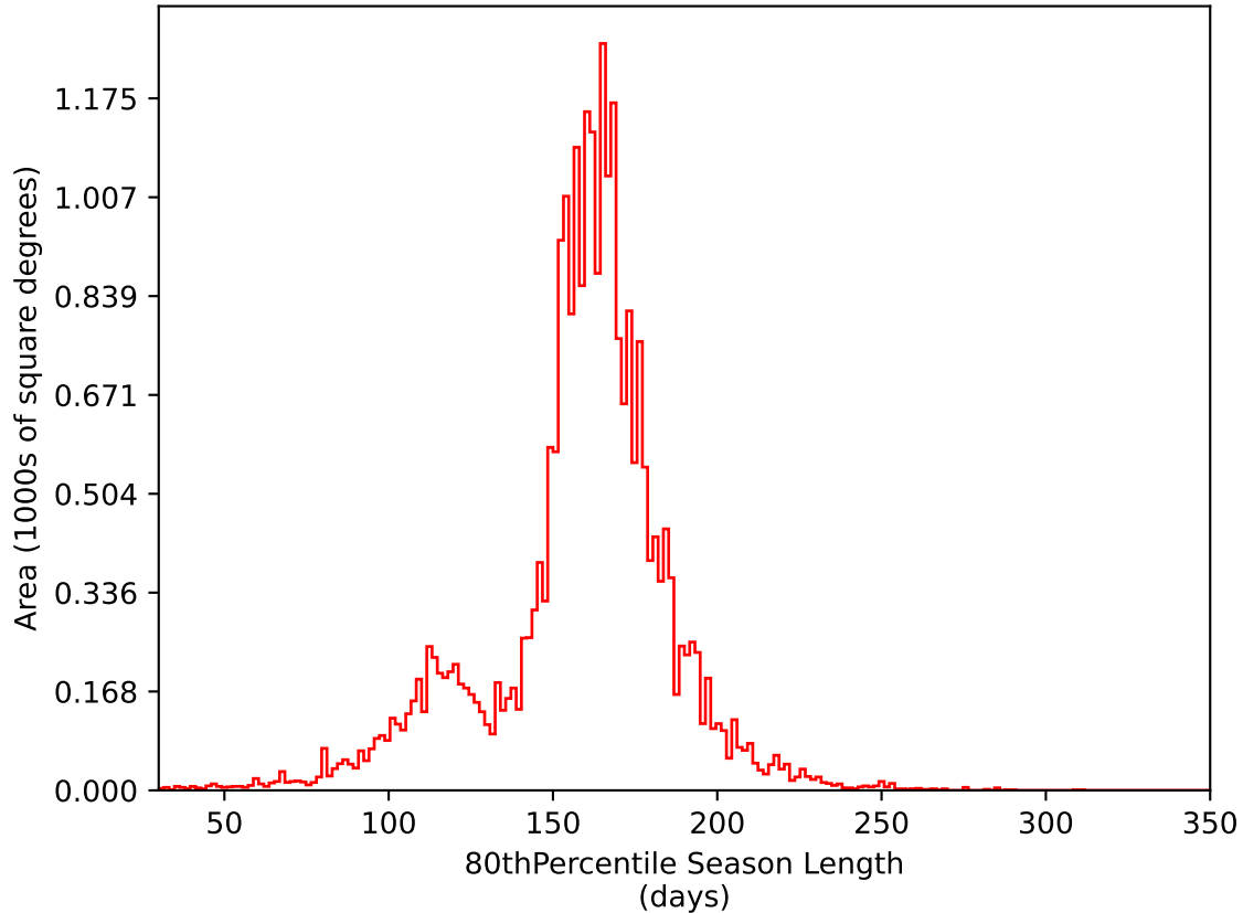
ddf_acor_sf25_lsf40_lsr10_v3.4_10yrs All sky i band: 80thPercentile Season Length
